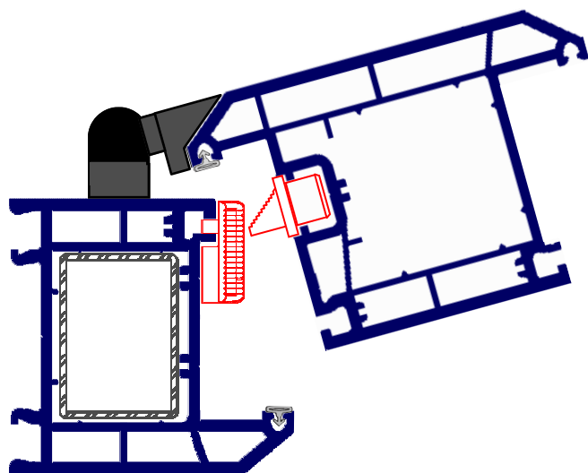
Frame Part
