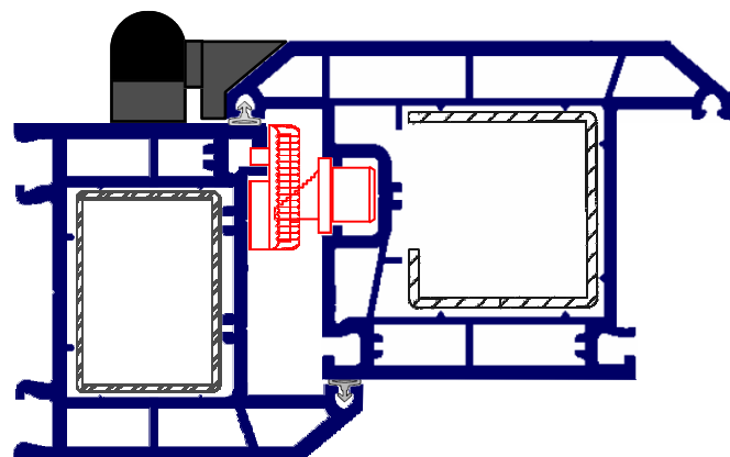
Section Through - Closed Position
