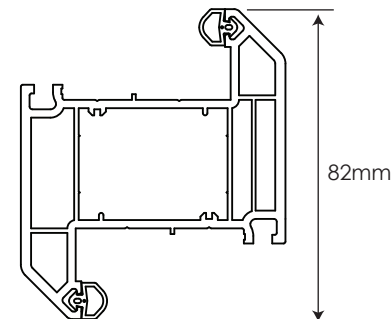
82mm Z Transom/Mullion 504605 / 584605
