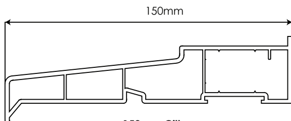
150mm Cill 504670 / 584670
