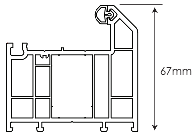
67mm Outerframe 504565 / 584565
