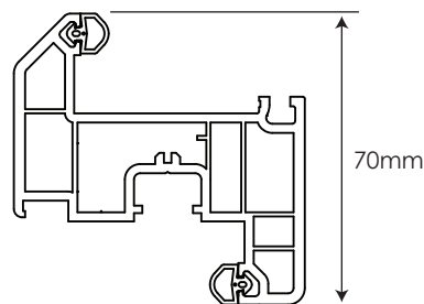
70mm Tilt/Turn Sash 504625 / 584625
