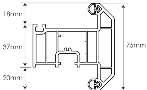
75mm Casement T Sash 504615 / 584615
