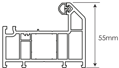
55mm Outerframe 504555 / 584555
