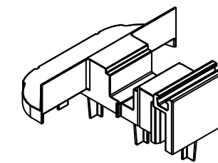
2888 Mullion End Cap French Flush Casement
