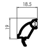
Ogee Glazing Bead 18.5mm 546572
