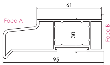
Stub Cill 95mm 246320
