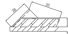
Weldable Corner Joint for Door Sash T + Z 259036
