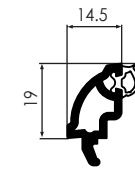
Ogee Glazing Bead 14.5mm for 32mm Sealed Units 503681
