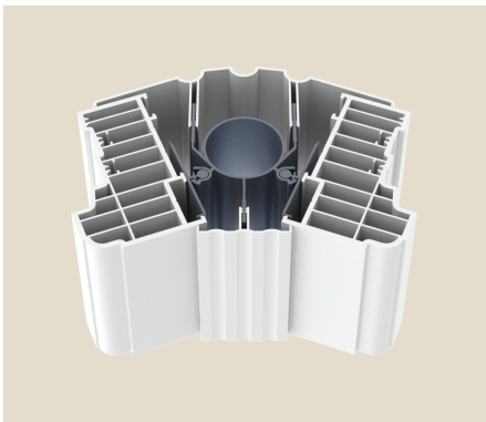
R109 120°-150° Variable Bay Post 482028 Frame Adapter PILDT, VSO Internal, External Trim Jack D VS
