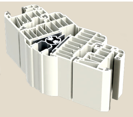
482055 150°-179° Variable Bay Post 482104 Frame Adapter DBI, DBO Internal, External Trim Jack C 482055
