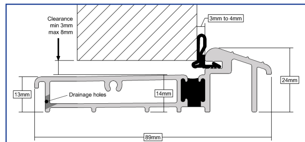
Stormguard AM5Ex78 Threshold Cill - Open Out Black Gasket Only - All uPVC Systems
