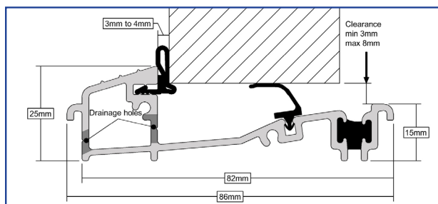
Stormguard AM3Ex78 Threshold Cill - Open In Black Gasket Only - All uPVC Systems
