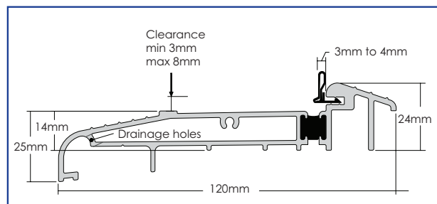
Stormguard AM5EX Threshold Sub Cill - Open Out Black Gasket Only - All uPVC Systems
