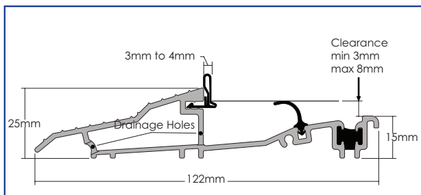
Stormguard AM3EX Threshold Cill - Open In Black Gasket Only - All uPVC Systems
