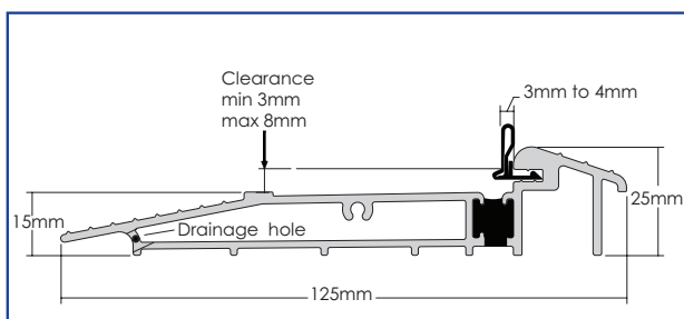
Stormguard AM5EX Threshold Cill - Open Out Black Gasket Only - All uPVC Systems
