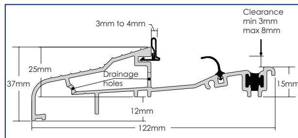
Stormguard AM3EX Threshold Sub Cill - Open In Black Gasket Only - All uPVC Systems
