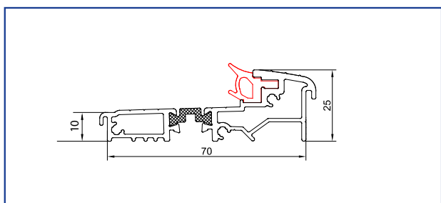
Exitex OUM 70 RITB Threshold - Open Out Black Gasket Only - Rehau Rio Only
