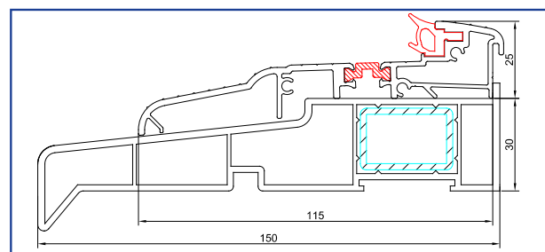
Exitex OUM 70 RITB Door Threshold Sub Cill - Open Out Black Gasket Only - Rehau Rio Only
