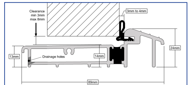
Stormguard AM5Ex 78 Threshold - Open Out Black Gasket Only - All uPVC Systems
