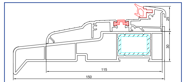
Exitex OUM 70 RITB Door Threshold Sub Cill - Open Out Black Gasket Only - Rehau Rio Only
