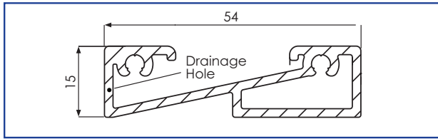
15mm Low Threshold Single Doors Only, White Gasket Only - Rehau and Calibre
