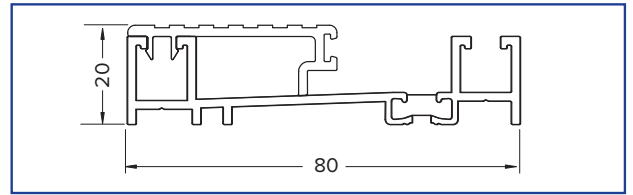
Low Threshold for Rehau Slinova Sliding Door Only External Ramp available
