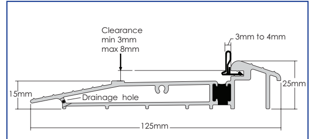
Stormguard AM5Ex 125 Threshold - Open Out Black Gasket Only - All uPVC Systems
