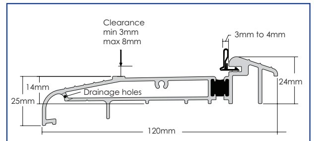
Stormguard AM5Ex 125 Threshold for cill - Open Out Black Gasket Only - All uPVC Systems
