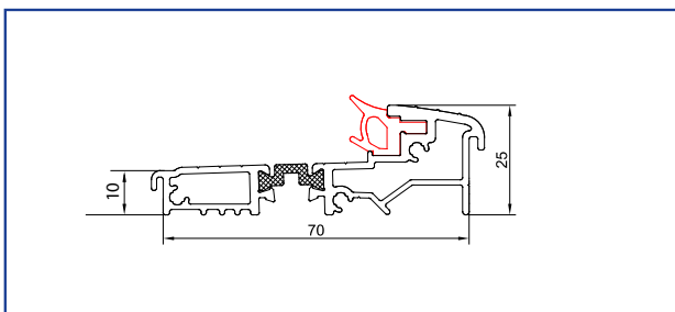
Exitex OUM 70 RITB Threshold - Open Out Black Gasket Only - Rehau Rio Only
