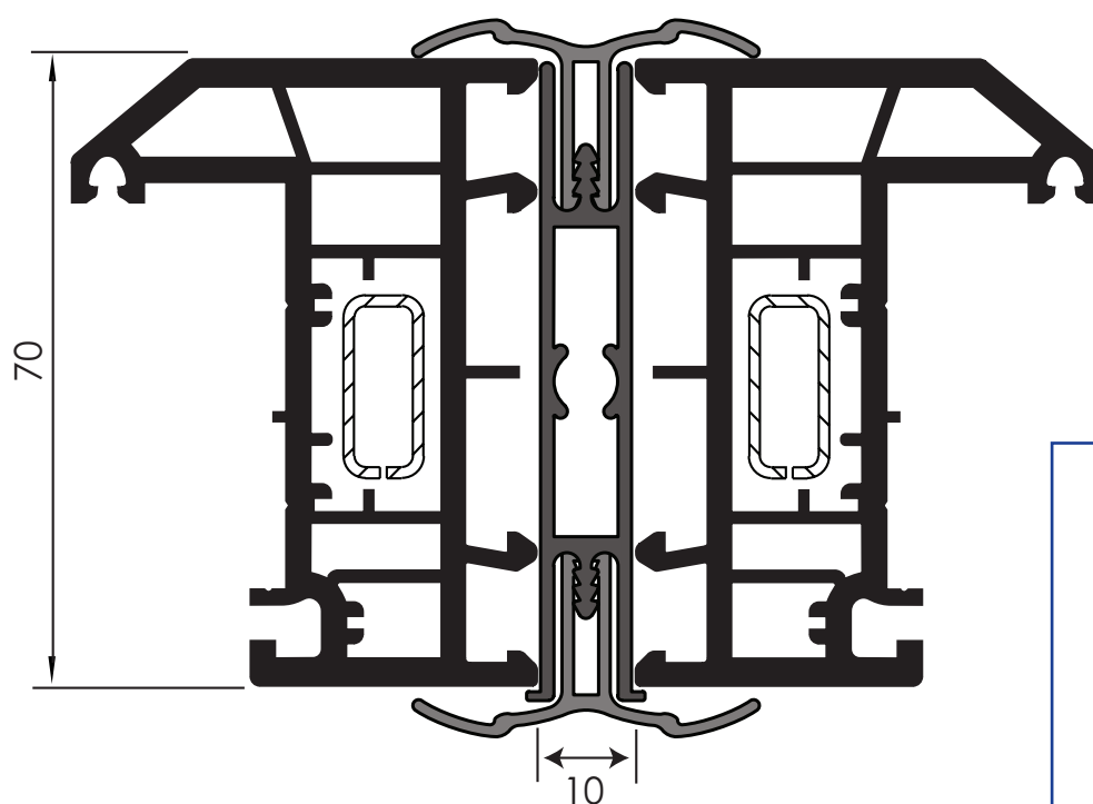
Bay jack for 10mm Coupler
