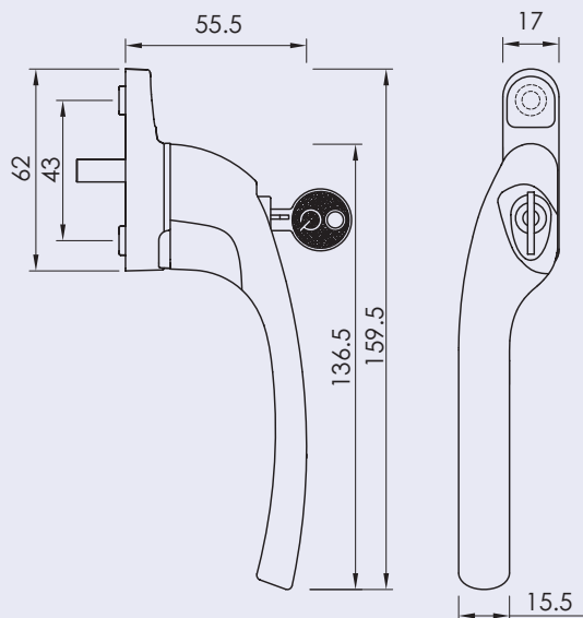
Alpha Left Crank Espag Handle with Cylinder
