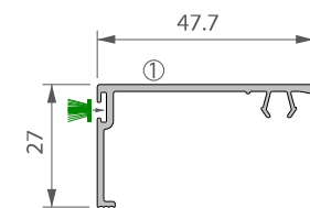
4456 COVER TRIM
