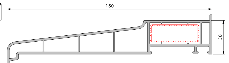
3339 - 180MM CILL
