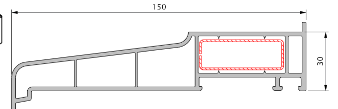
3338 - 150MM CILL
