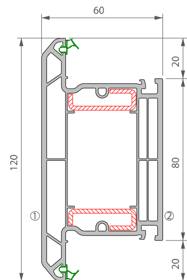
4435 - MIDRAIL
