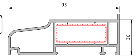
3337 - 95MM CILL
