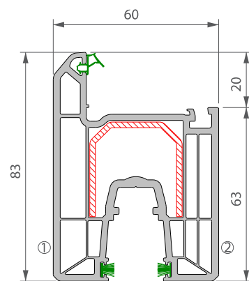
4410 - SASH
