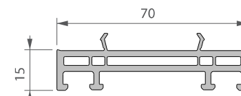
3336 - 15MM ADD-ON
