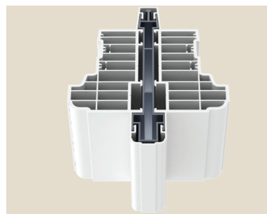
R7120 10mm In-Line Coupler R204 Internal Trim R203 External Trim
