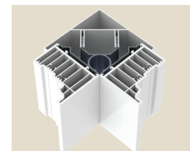
R78108 90° Corner Post 90SQ Square Corner Post Cover Jack D WWL142
