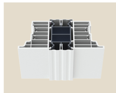
482055 160°-180° Variable Bay Post 482104 Frame Adapter DBI, DBO Internal, External Trim Jack C 482055
