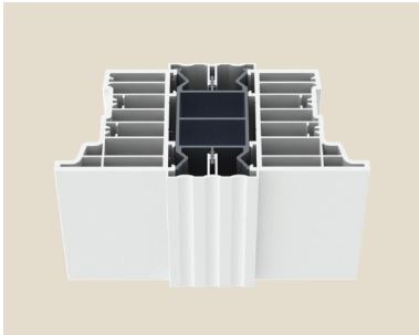
482055 160°-180° Variable Bay Post 482104 Frame Adapter DBI, DBO Internal, External Trim Jack 19
