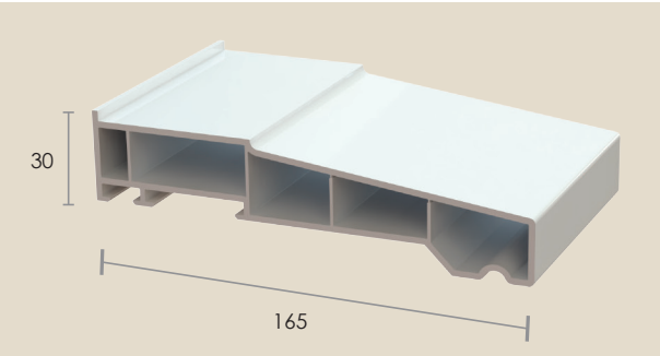
R217 Internal Cill Trims - use with R007, R008, R009M R214 Internal Cill Trim - use with R009
