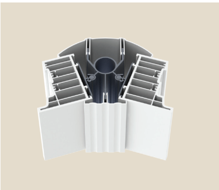
R7109 120°-165° Variable Bay Post 482028 Frame Adapter PILDT, DBO120 Internal, External Trim Jack 18
