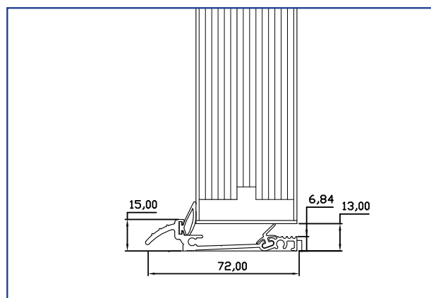
Macclex Aluminium Threshold Cill - Open In/out
