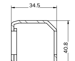
361488 REINFORCEMENT 34.1 X 40.8 X 2MM
